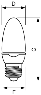
Candle 8W/827 E27 220-240V 50/60Hz
